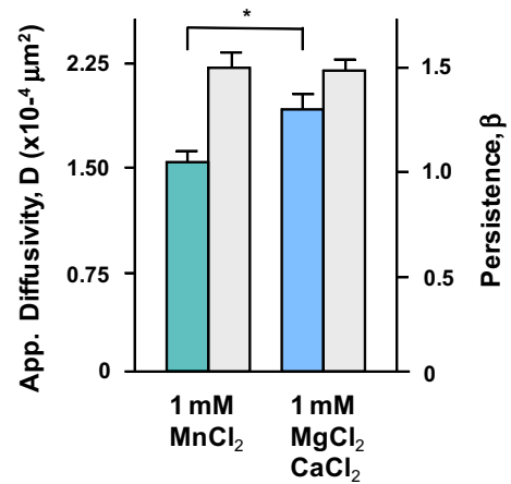
Fig. 4. The apparent diffusivity of RGD-coated beads on K562 cells upon treatment with 1 mM \text{Mn}^{2+} and \text{Ca}^{2+}/\text{Mg}^{2+} ions. \text{Mn}^{2+} -treated cells (activated integrin, green) show a tighter link of the integrin-FA-cytoskeleton connection than \text{Ca}^{2+}/\text{Mg}^{2+} -treated cells (inactive integrin, blue), whilst the persistence (gray) remained similar (superdiffusive) for both \text{Mn}^{2+} - and \text{Mg}^{2+}/\text{Ca}^{2+} ion treated cells. Note, that the bead motion only reflects the dynamics of the cytoskeleton as long as the bead is connected. The number of cells analyzed were between 750 and 950; number of experiments n = 5 . (*) indicates statistically significant data. (For interpretation of the references to colour in this figure legend, the reader is referred to the web version of this article.)
