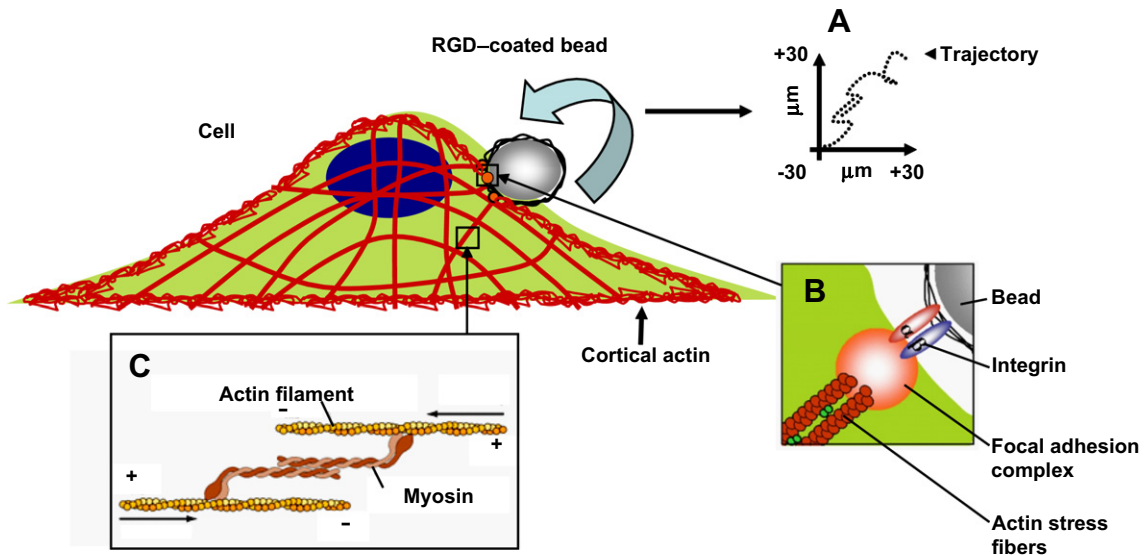
Fig. 2. Schematic representation of a 4.5\ \mu\text{m} Ø RGD-coated polystyrene bead attached to integrins of K562 cells that span the cell membrane. Integrins are connected via focal adhesions to the actin cytoskeleton. The insets show (A) the movement (trajectory) of a bead attached to the integrin receptor over 10 min, (B) the integrin-FA-cytoskeleton link, and (C) the contractile apparatus of the cell.
